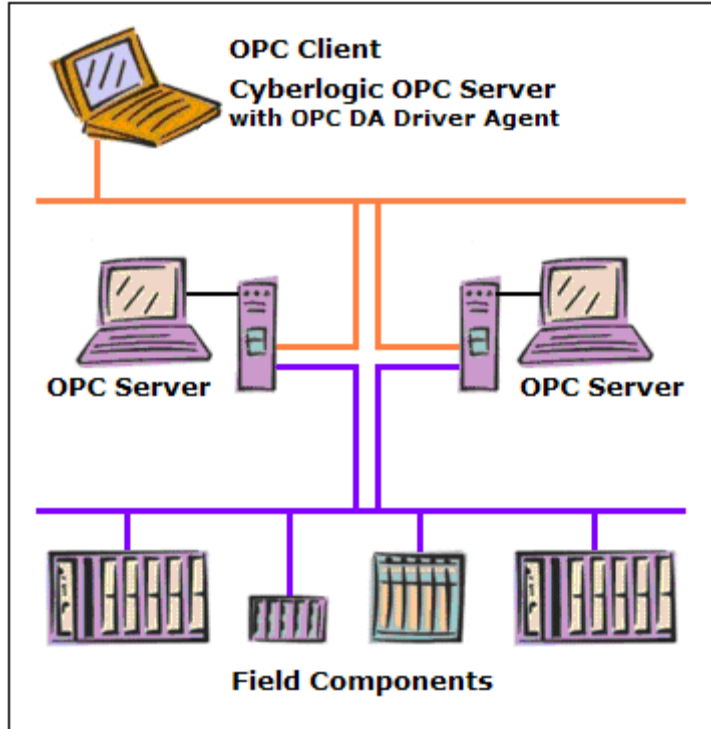
Cyberlogic's OPC DA Driver Agent lets you set up redundant OPC servers for greater reliability
