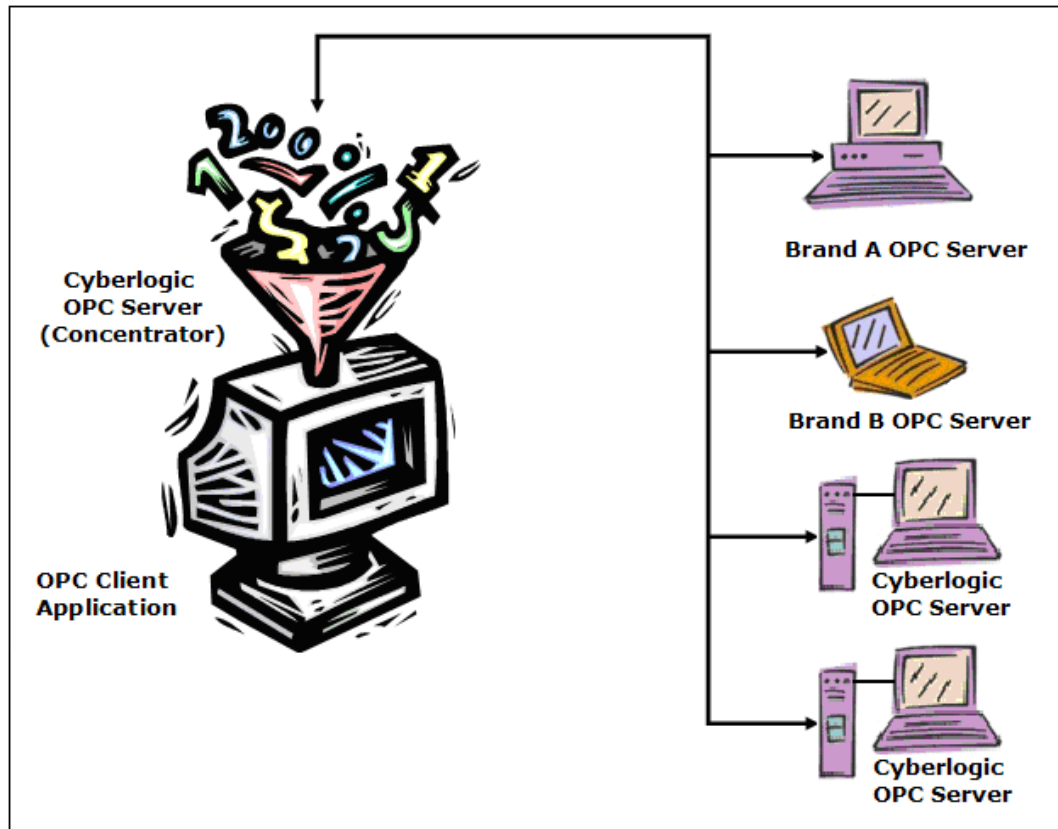
A Cyberlogic OPC Server connects to several other OPC servers, providing a single access point for all of the data.
